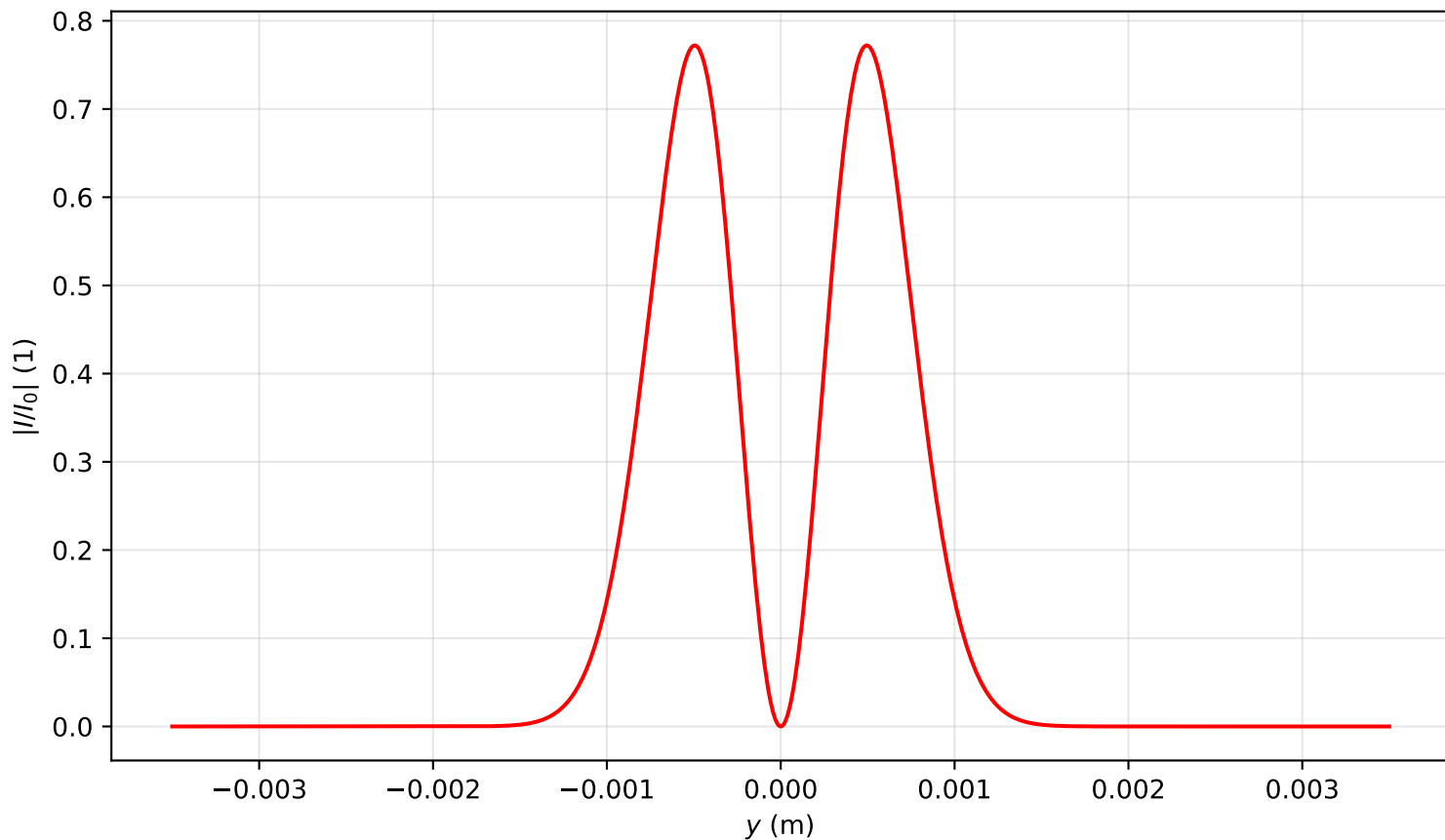
Intensity profile I(x=0, y, z=0.080)/I_0 , P_{in}=2.0P_{cr} , artificial time
